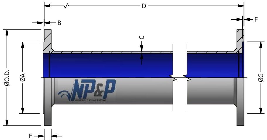
MALE FLANGE
