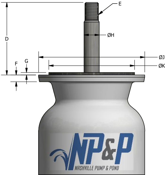
BOWL/DISCHARGE DIMENSIONS
